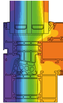
Distribution of isotherms in MB-79N SI window
