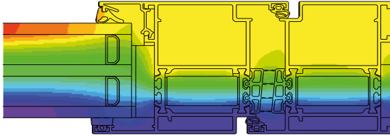
Distribution of isotherms in MB-79N SI+ door
